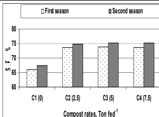
Fig. (2): Effect of compost rates on structure factor in the two seasons
