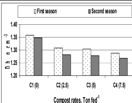
Fig. (1): Effect of compost rates on soil bulk density in the two seasons
